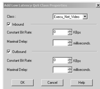
Low Latency QoS Class Properties
